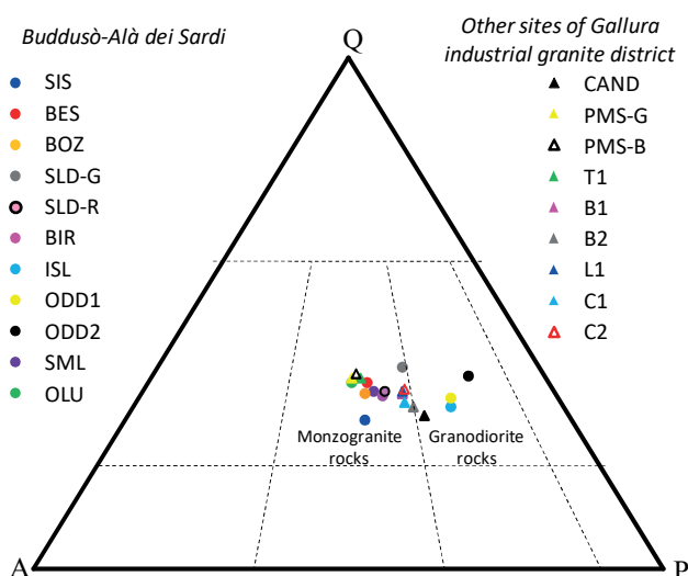
FIGURE 4: Classification of the sampled rocks (Cerri et al., n.d.). Q: quartz; A: sum of Na- and K-feldspar; P: plagioclase.
