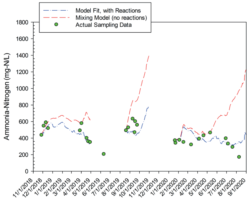
FIGURE 3: Fit of ammonia-nitrogen concentrations with volatilization and nitrification and concentrations computed from a mixing only model (e.g., no reactions occurring).
